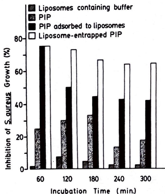
FIG. 1. Percentages of S. aureus growth inhibition, expressed as [(\text{optical density of control minus optical density of sample})/(\text{optical density of control})] \times 100 , determined at different time points. Each bar represents the arithmetic mean of triplicates from a typical experiment.
