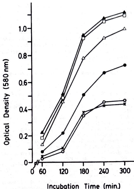
FIG. 2. S. aureus growth, measured as optical density of the cultures at different time points. S. aureus was grown in the following media: ▲, medium alone; □, PIP (50% MIC) + exogenous \beta -lactamase; △, PIP (50% MIC); ●, PIP adsorbed to liposomes; ○, liposome-encapsulated PIP + exogenous \beta -lactamase; and ×, liposome-encapsulated PIP. Each point represents the arithmetic mean of triplicates from a typical experiment.
